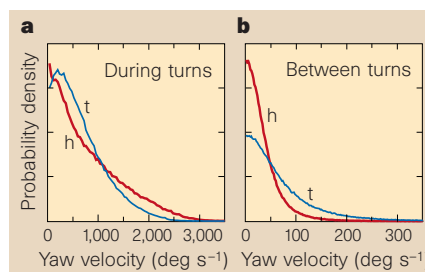
Figure 2 Gaze stabilization between turns. a , Probability densities of yaw velocities during turns, showing that yaw velocities of the head (h) reach higher values than those of the thorax (t). Total flight time was 703 seconds by four flies, during which time 6,697 turns were made. b , Between turns, yaw velocities of the head are significantly lower than those of the thorax, and both are much lower than during turns. More detailed figure legends are available as Supplementary information.
