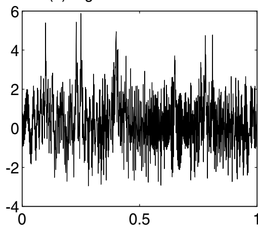
(a) Signal: Werner Sorrows
