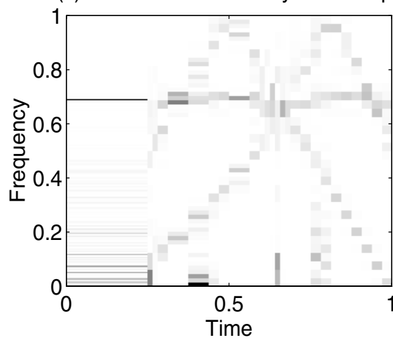
(c) Phase Plane: BOB by \ell^1 Entropy
