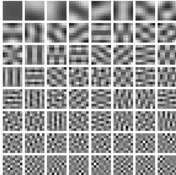
Figure 1: Principal components calculated on 8 \times 8 image patches extracted from natural scenes using Sanger’s rule [14]. The full set of 64 components are shown, ordered by their variance (by columns, then by rows). The oriented structure of the first few principal components does not arise as a result of the oriented structures in natural images, but rather because these functions are composed of a small number of low frequency components (the lowest spatial frequencies account for the greatest part of the variance in natural scenes [8]). Reconstructions based solely on the first row of functions will merely yield blurry images. Identical looking components are obtained for images with the same amplitude spectrum as natural images but with randomized phases (i.e., 1/f noise).
